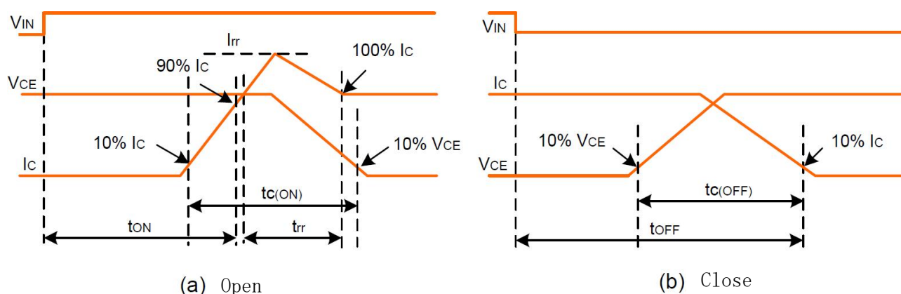
Figure 1 Definition of switching time
